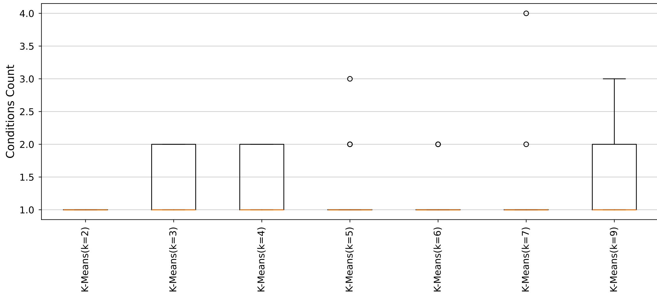
YARA Rules Conditions Count Distribution (Cluster12_Size9 dataset)
